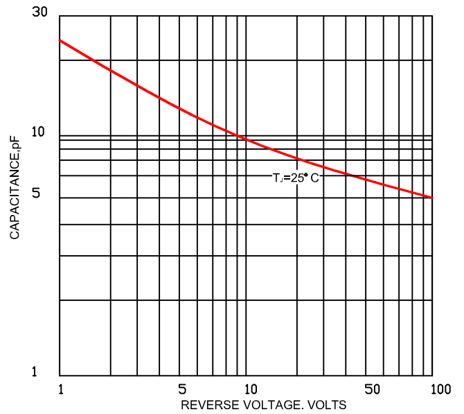
FIG.4-TYPICAL REVERS CHARACTERISTICS
